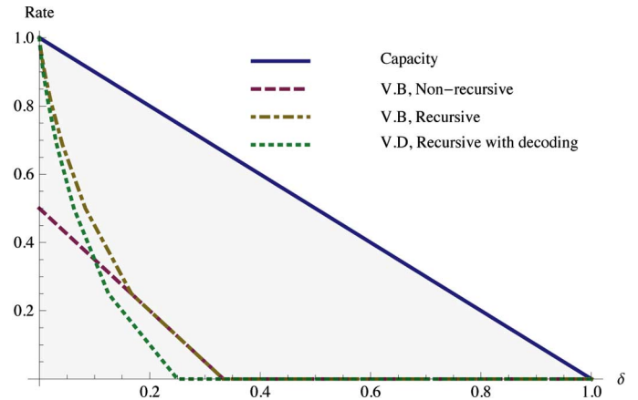
Fig. 5. Asymptotic rate versus distance for several code constructions. The horizontal axis is \delta = \lim \frac{d(n)}{n} .
